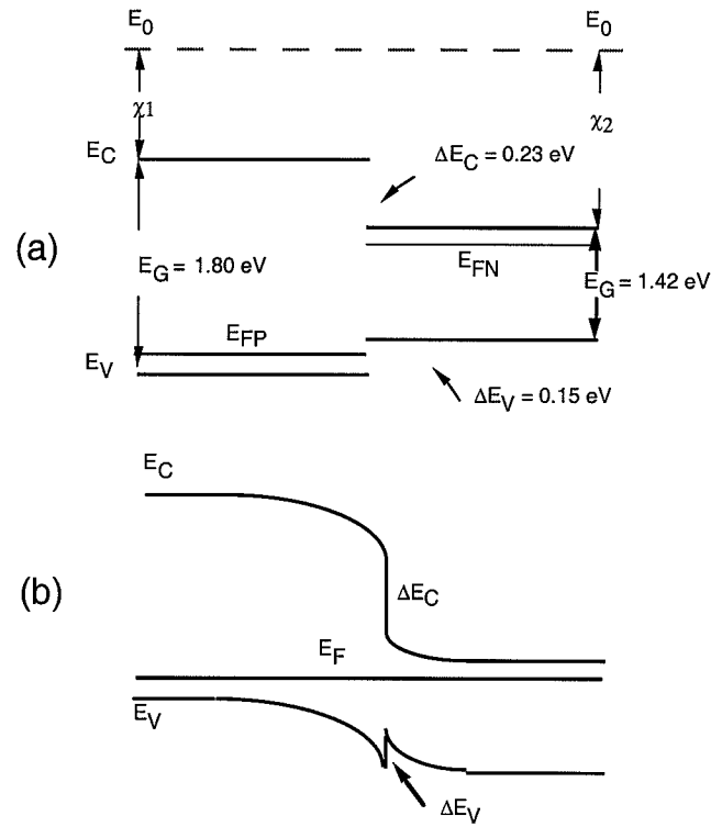
Fig. 6. \text{Al}_{0.3}\text{Ga}_{0.7}\text{As} : \text{GaAs} P-n heterojunction. (a) before contact. (b) after contact.
