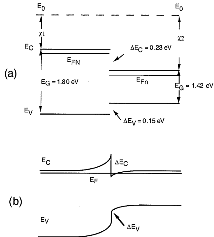
Fig. 7. \text{Al}_{0.3}\text{Ga}_{0.7}\text{As} : \text{GaAs} N-n heterojunction. (a) before contact. (b) after contact.
