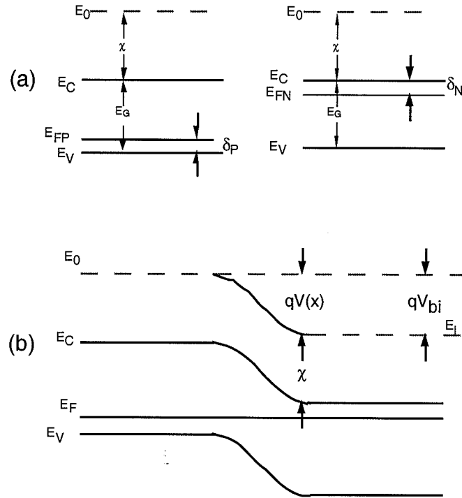
Fig. 2. Illustration of the formation of a pn junction. (a) the isolated semiconductors are characterized by separate Fermi levels, and (b) after placing them in contact, electrons flow from the region with the higher Fermi level to the region with the lower Fermi level. As a result of this flow, a space-charge layer builds up and a built-in potential results. In equilibrium, the final structure is characterized by a single Fermi level. Note that E_0 is lowered to E_l(x) , the local vacuum level.
