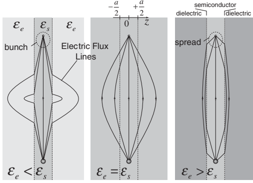
FIG. 1. Electric flux lines originating from a fixed ionized impurity and terminating on a mobile electron, and the effect of the dielectric environment. The flux lines bunch closer inside the semiconductor layer if \epsilon_e < \epsilon_s , and spread farther apart if \epsilon_e > \epsilon_s , thus enhancing Coulomb interaction in the former case and damping it in the latter.
