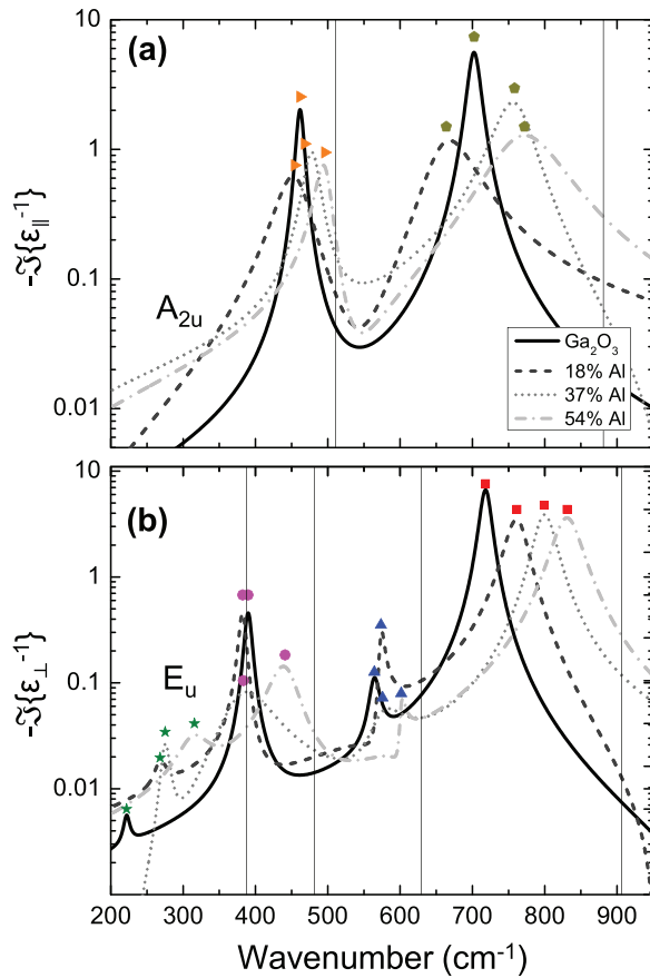
FIG. 2. The negative imaginary part of the inverse dielectric functions for all samples investigated here. (a) \Im\{-\epsilon_{\parallel}^{-1}\} and (b) \Im\{-\epsilon_{\perp}^{-1}\} . Data for \alpha\text{-Ga}_2\text{O}_3 are included for comparison. Vertical lines indicate LO frequencies for \alpha\text{-Al}_2\text{O}_3 . Symbols indicate peak positions and, thereby, LO modes of the ternary alloys.
