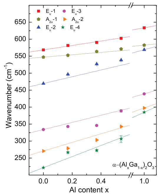
FIG. 3. Best match model calculated phonon mode parameters (TO; symbols) for all observed phonon modes for the \alpha\text{-(Al}_x\text{Ga}_{1-x})_2\text{O}_3 thin films. Lines are linear interpolations between corresponding phonon modes of the binary compounds. Error bars are included on each data point, though many are too small to be seen behind the symbol.
