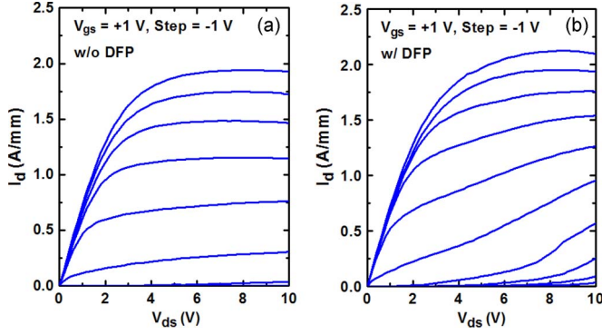
Fig. 1. Common-source family of I_d - V_{ds} 's (a) before and (b) after DFP on the device with L_g = 60 nm and L_{sdl} = 1.6 \mu m.
