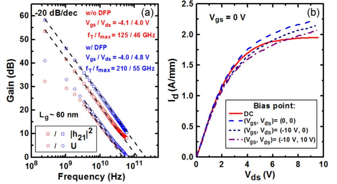
Fig. 3. (a) Current gain and unilateral gain of the device, showing f_T/f_{max} = 125/46 and 210/55 GHz before and after DFP, respectively. (b) Pulsed I - V measurements after DFP, with a 300-ns pulsewidth and a 0.5-ms period.
